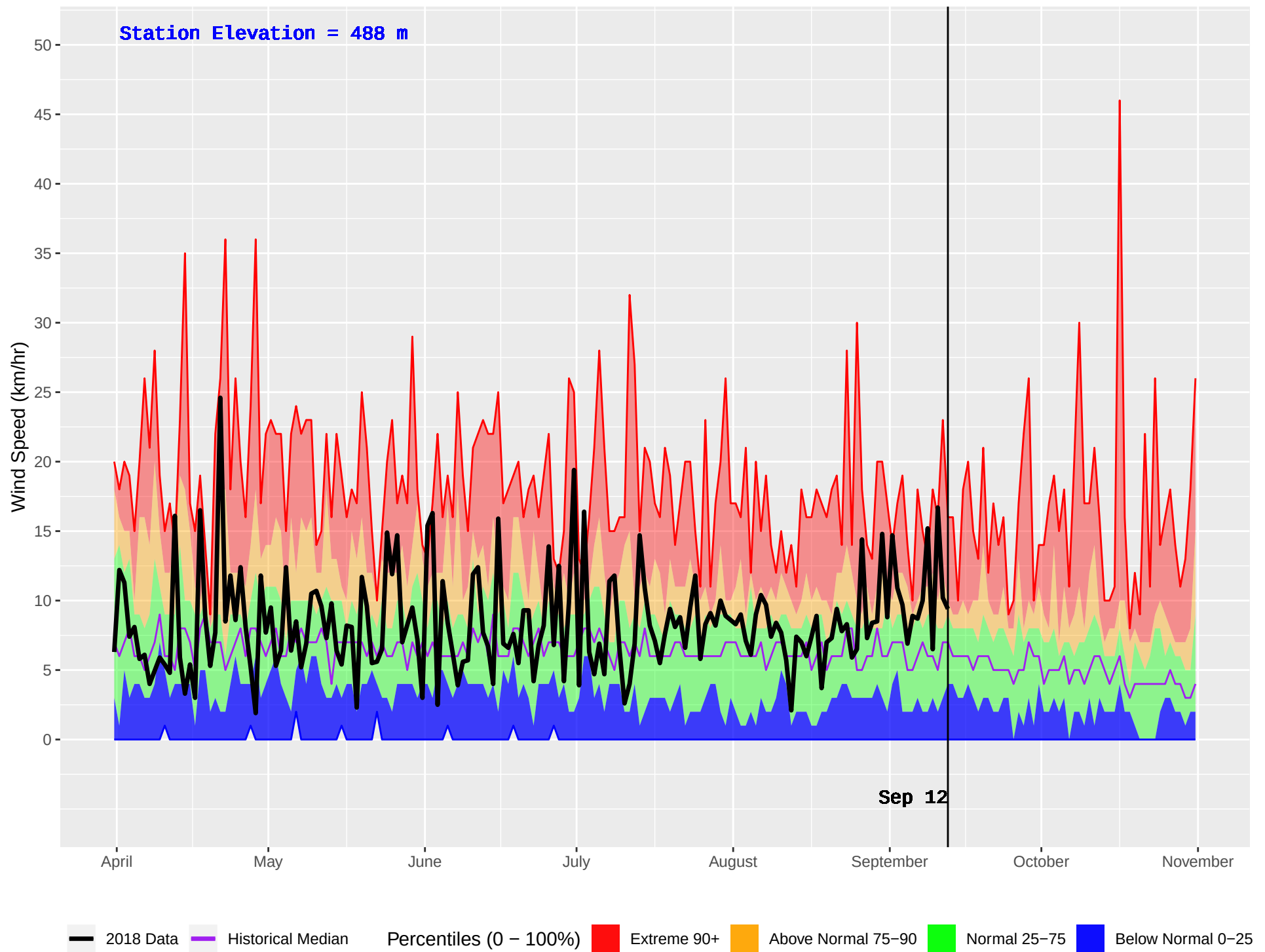
MABEL LAKE 2 (362) : Historical (1987–2016) and Current (2018) Daily Wind Speed
